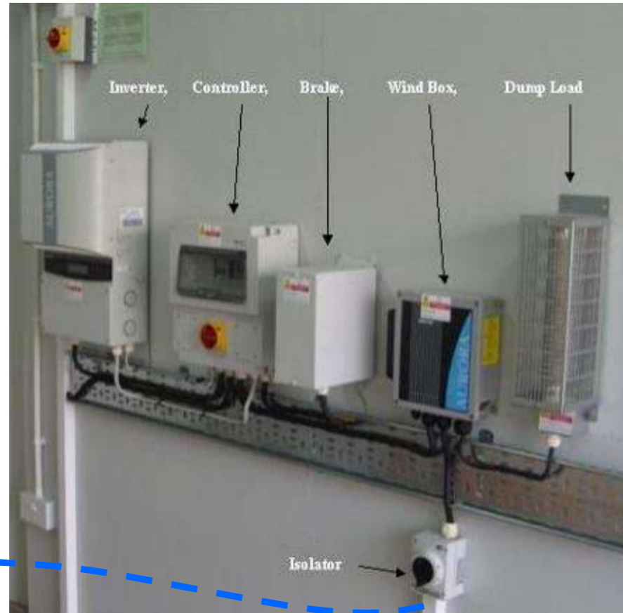
Equipment required along with the tower and turbine
